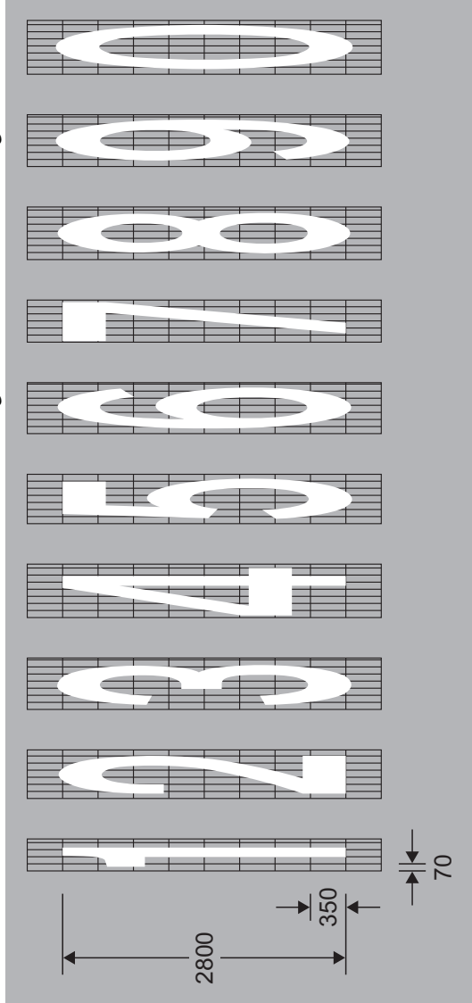
Letters, numerals and other characters for use in road markings where the character height is 2800 mm
